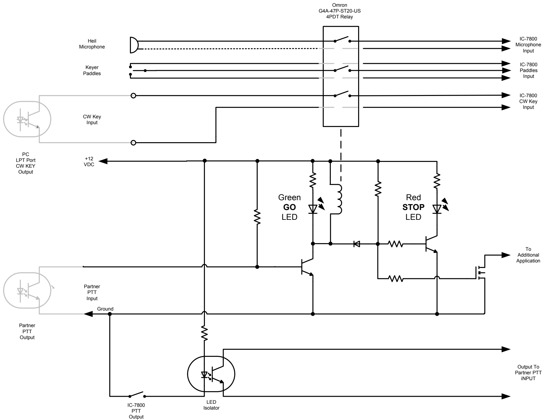
K3LR Interlock Circuit 29 Sep 2011
